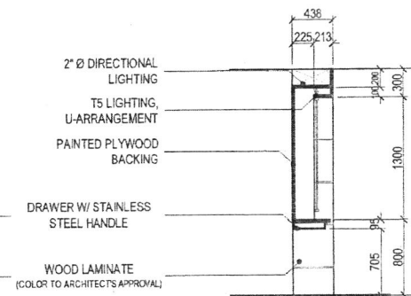
SECTION THRU "A"
