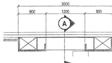
BLOW - UP PLAN
