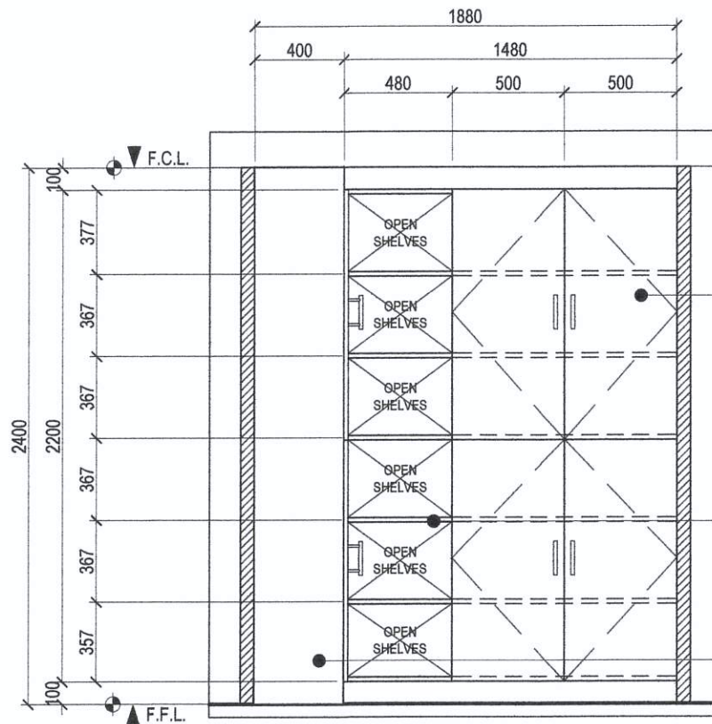
ELEVATION 'A'
