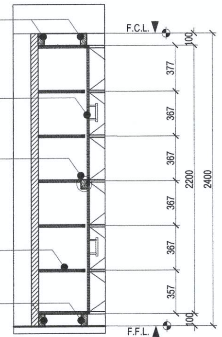
SECTION 'C'
