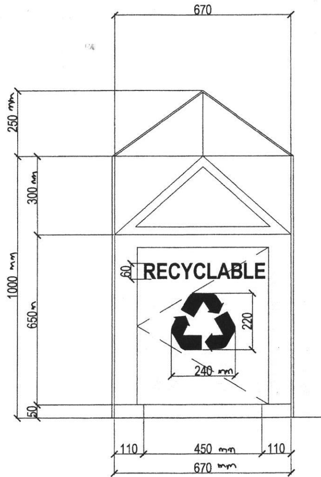
FRONT VIEW
