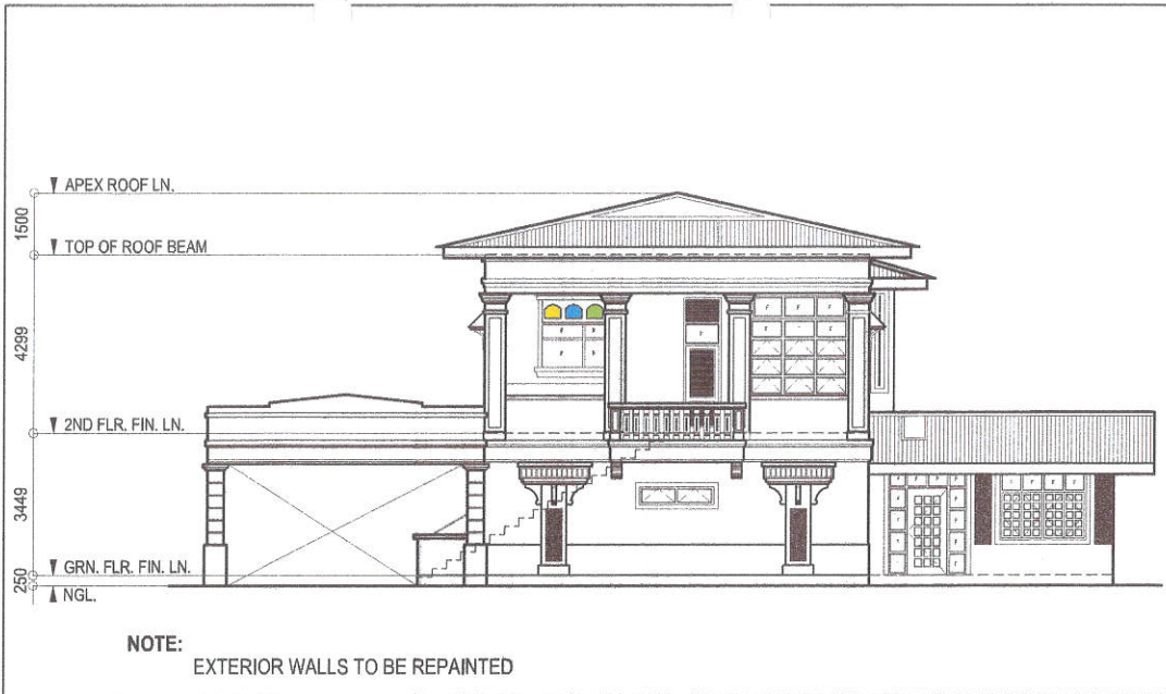
1 FRONT ELEVATION - HERITAGE HOUSE
