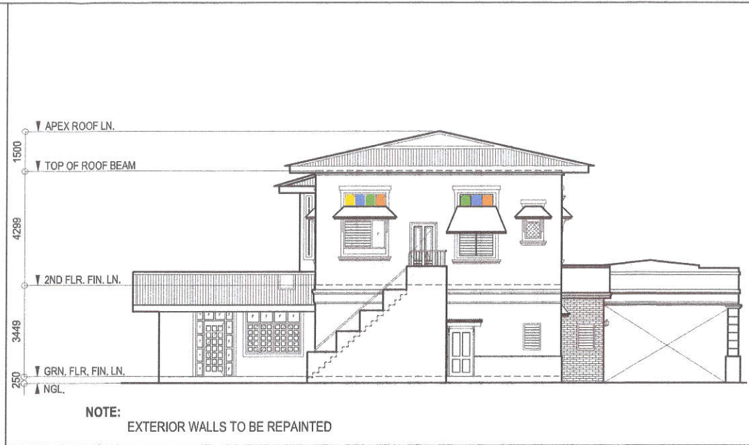
2 REAR ELEVATION - HERITAGE HOUSE
