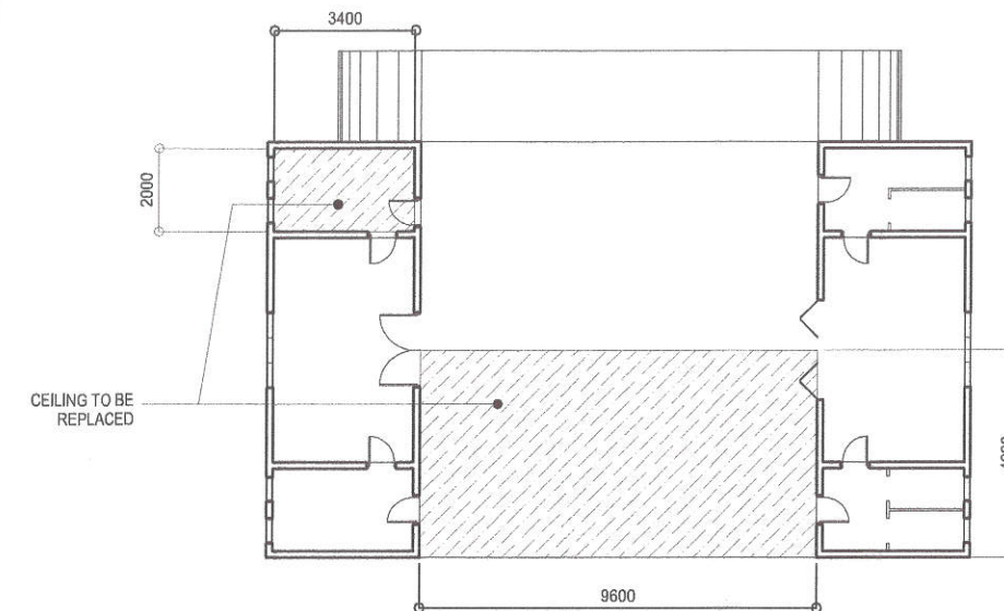
3 GROUND FLOOR REFLECTED CEILING PLAN - SOCIAL HALL
