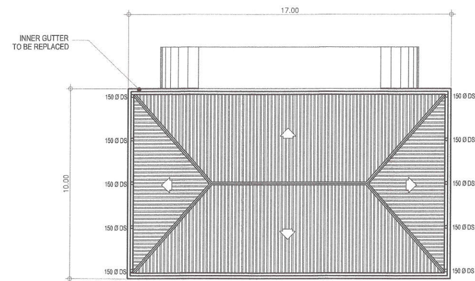
3 ROOF STORM DRAINAGE LAYOUT- SOCIAL HALL
