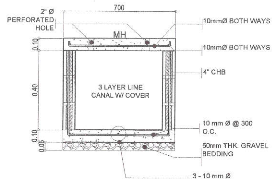
1 TYPICAL DETAIL FOR 3-LAYER LINED CANAL
