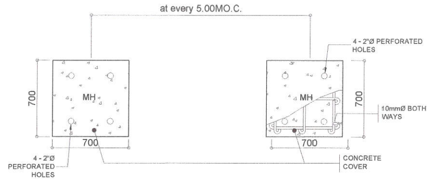
2 3 LAYER LINED CANAL CONCRETE COVER DETAIL
