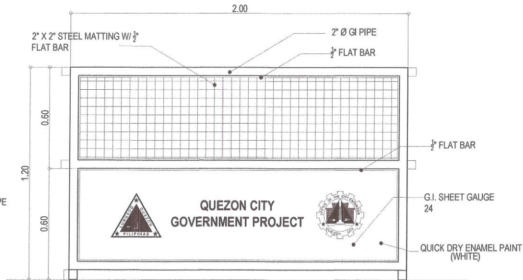
FRONT VIEW
