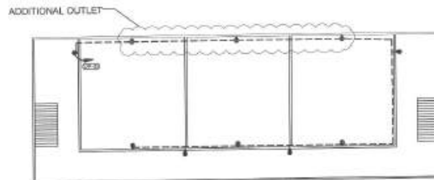
3 GROUND FLOOR POWER LAYOUT (BUILDING 3)
