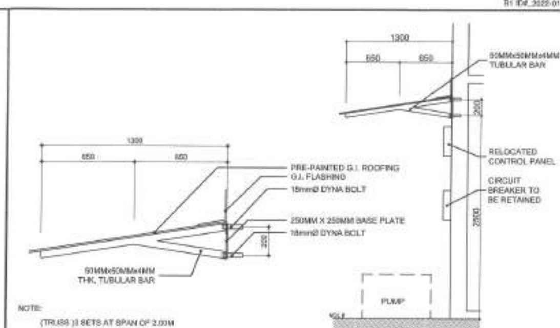
3 CANOPY DETAIL
