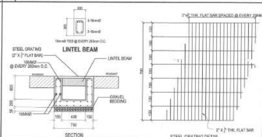
4 DRAINAGE INTERCEPTOR DETAIL
