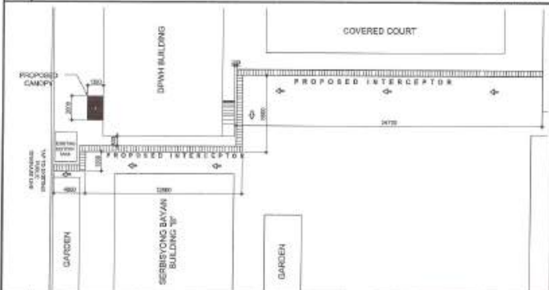
2 PROPOSED DRAINAGE INTERCEPTOR LAYOUT PLAN
