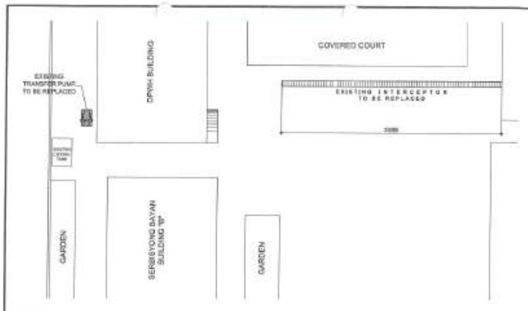
1 EXISTING DRAINAGE LAYOUT PLAN
