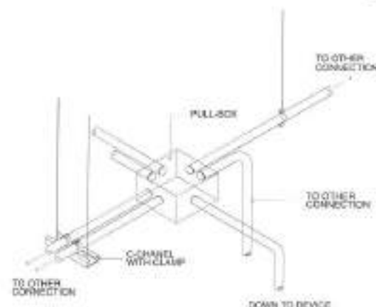
SPOT DETAIL OF CONDUIT RUN AND BOX
