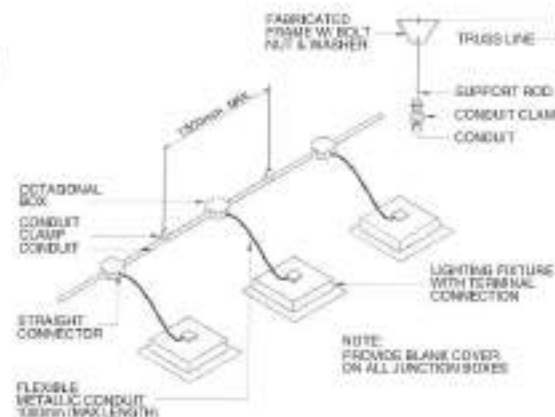
CONDUIT RUN FOR LIGHTING DISTRIBUTION IN ONE CIRCUIT (FOR EXPOSED OR INSIDE DROP-CEILING INSTALLATION)
