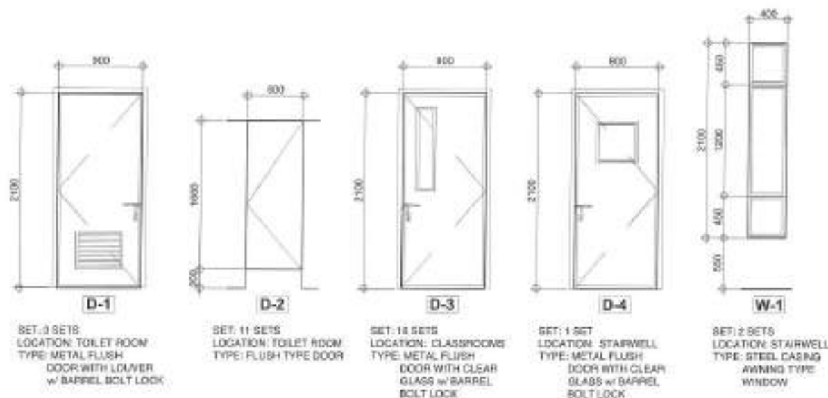
2 SCHEDULE OF DOORS & WINDOWS
