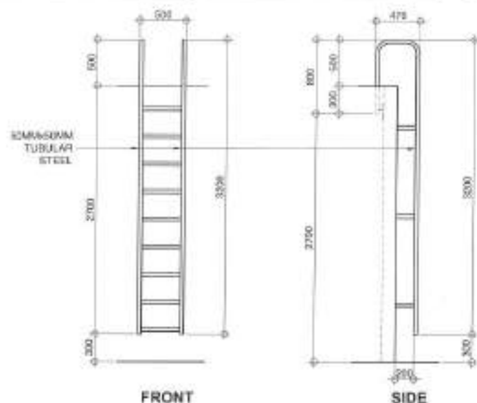
3 STEEL LADDER DETAILS (AT ROOF DECK)
