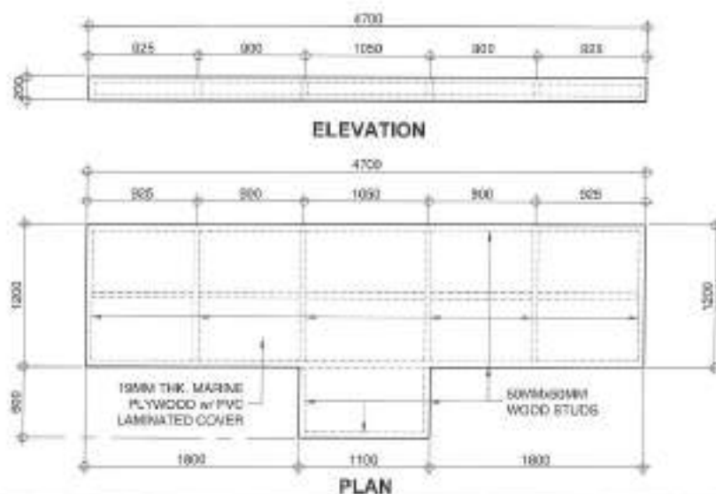
1 PLATFORM DETAILS (SECOND FLOOR AT SCIENCE LABORATORY)
