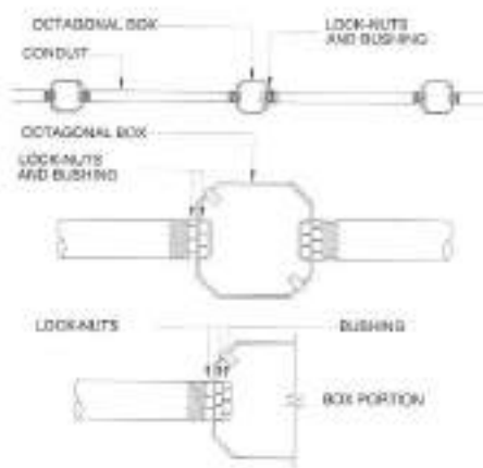
SPOT DETAIL OF CONDUIT RUN AND BOX
