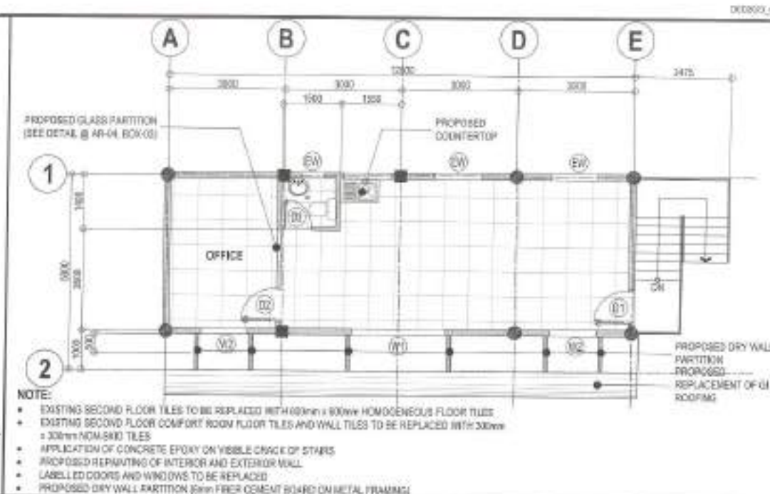
2 PROPOSED SECOND FLOOR PLAN
