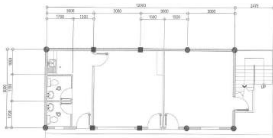
1 GROUND FLOOR LIGHTING LAYOUT
