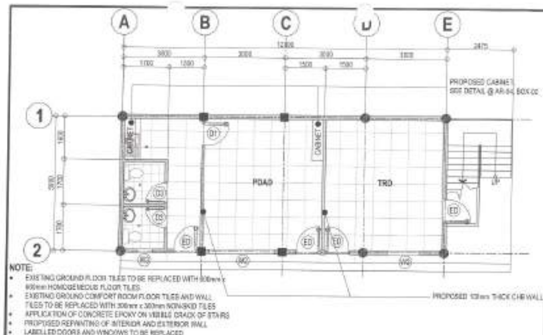
1 PROPOSED GROUND FLOOR PLAN
