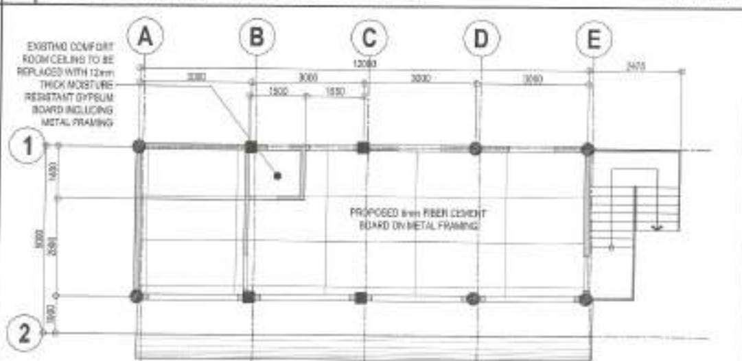
4 SECOND FLOOR REFLECTED PLAN
