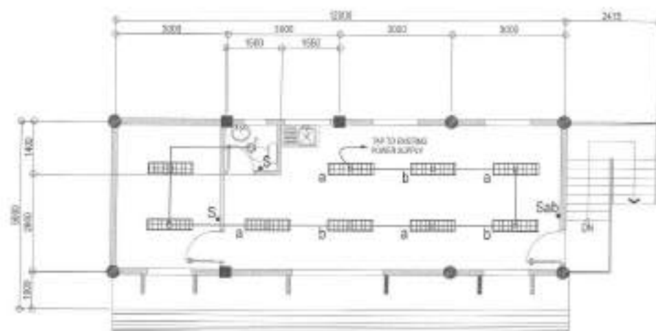
2 SECOND FLOOR LIGHTING LAYOUT
