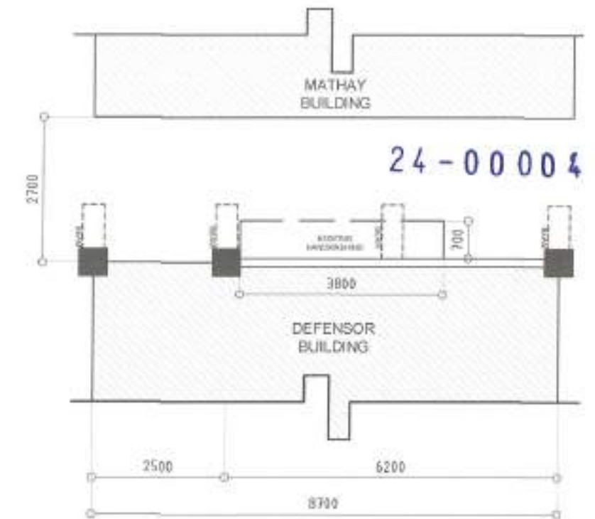
3 HWF 2 FLOOR PLAN
