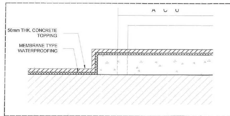
ACU CONNECTING TO CONCRETE SLAB SPOT DETAIL
