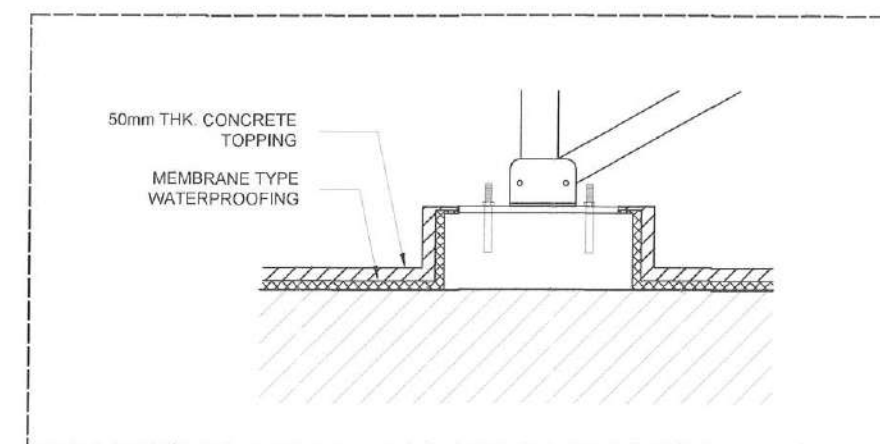
SOLAR PANEL CONNECTING TO CONCRETE SLAB SPOT DETAIL
