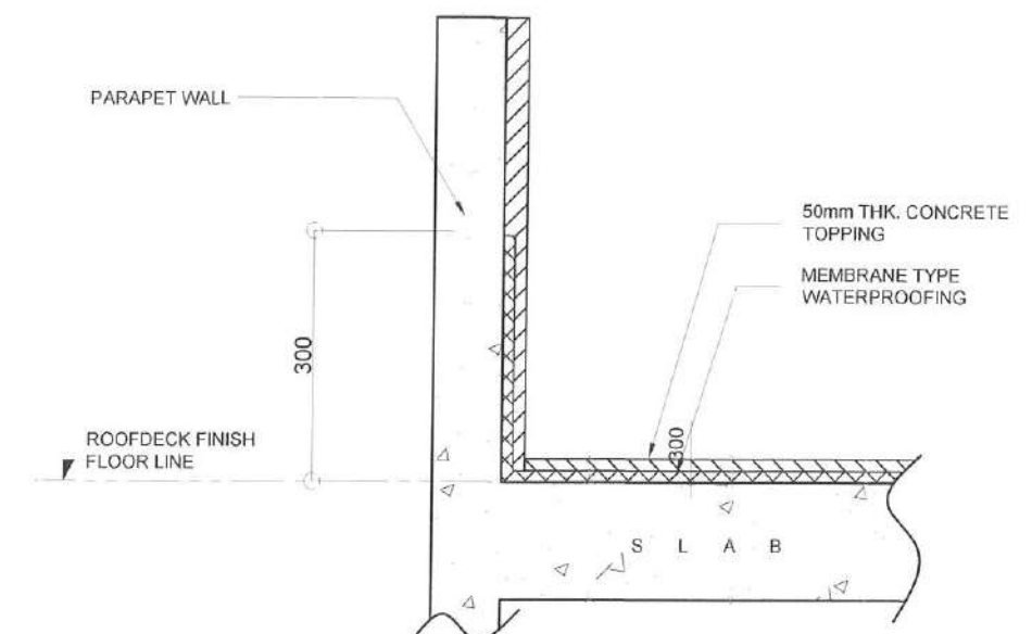
SLAB SECTION DETAIL
