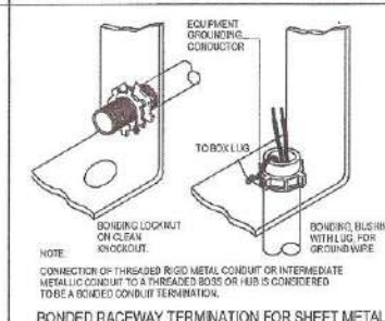
BONDED RACEWAY TERMINATION FOR SHEET METAL
