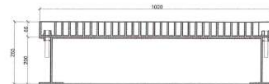
GRATING ELEVATION
