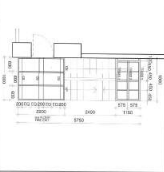
3 FIRE EXIT STAIR (RIGHT SIDE) 3RD FLR FRAMING PLAN SCALE: 1/75
