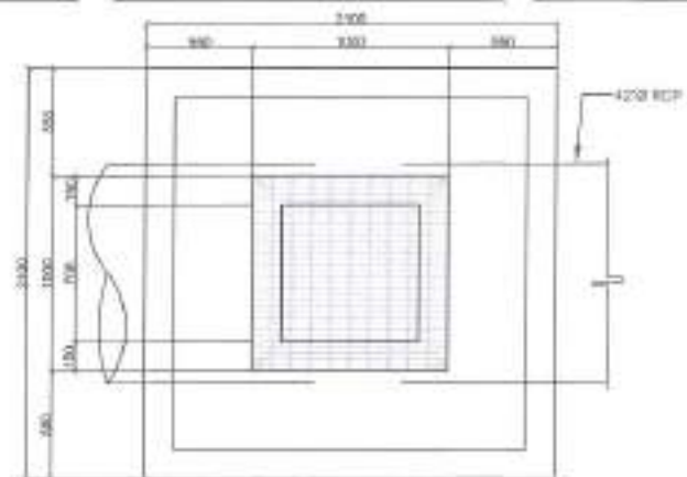
INTERCEPTOR PLAN
