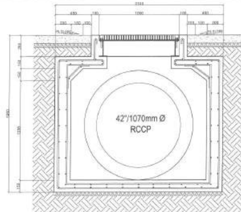
ELEVATION SECTION
