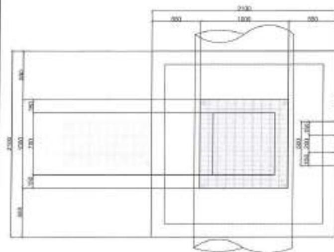
INTERCEPTOR PLAN SCALE: 1:30MTS
