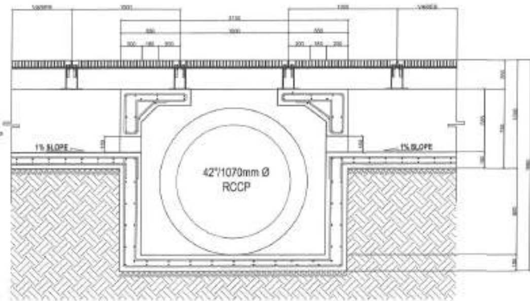
ELEVATION SECTION SCALE: 1:25MTS
