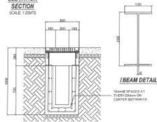
ELEVATION SECTION SCALE: 1:25MTS
