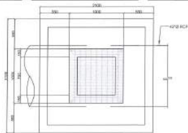
INTERCEPTOR PLAN
