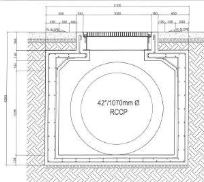
ELEVATION SECTION
