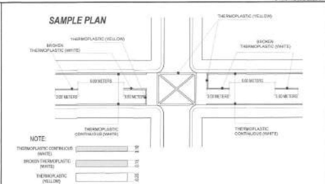
2 THERMO PLASTIC DETAIL
