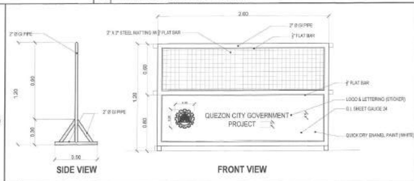
4 ROAD SAFETY BARRIER SYSTEM (STEEL BARRICADE) DETAIL
