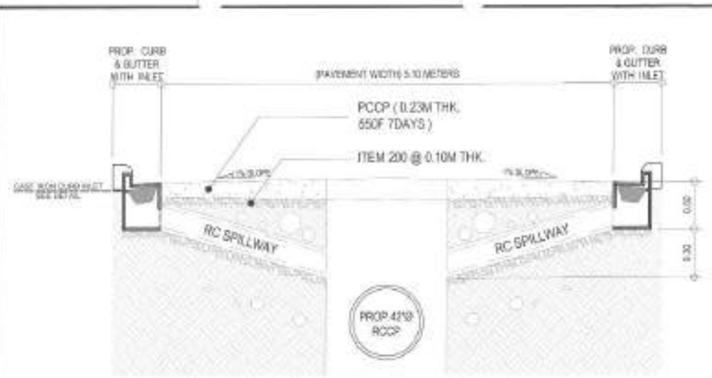
1 ROADWAY SECTION A
