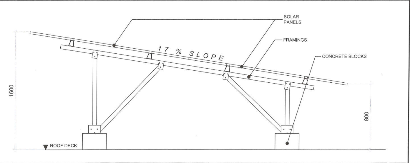
SOLAR PANEL DETAIL (CIVIC CENTER BUILDING F)
