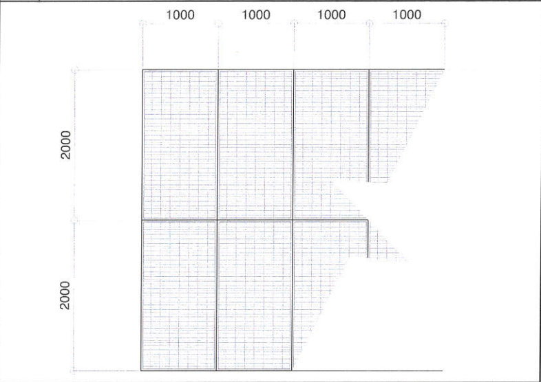
SOLAR PANEL PLAN (CIVIC CENTER BUILDING F)
