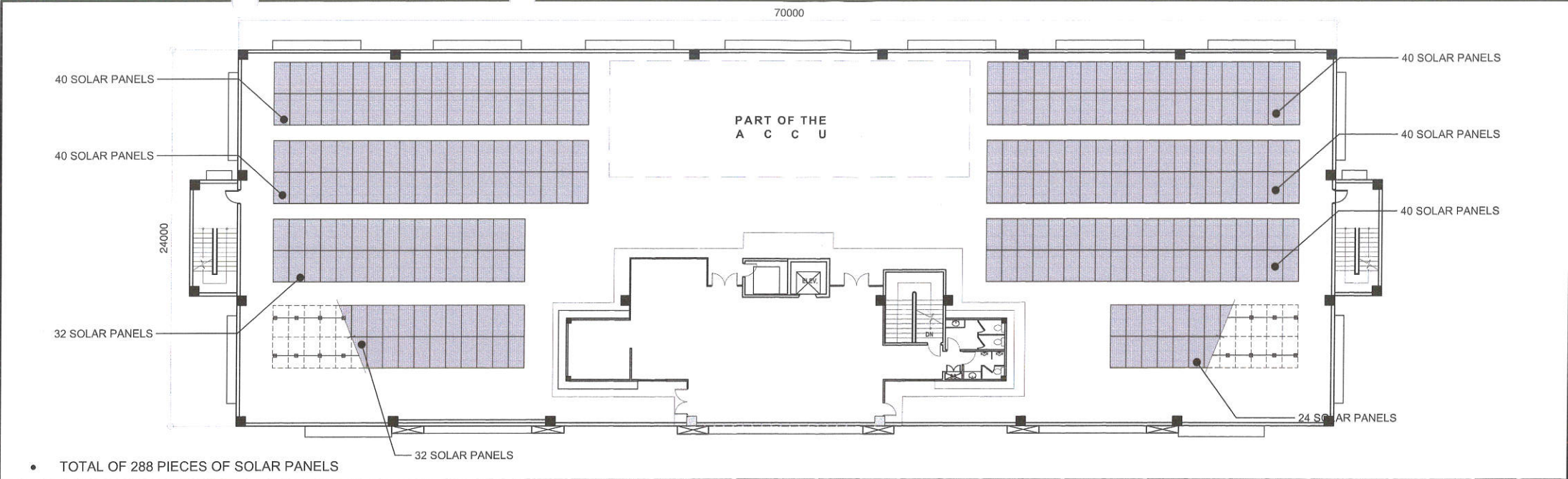
SOLAR PANEL LAYOUT (CIVIC CENTER BUILDING F)
