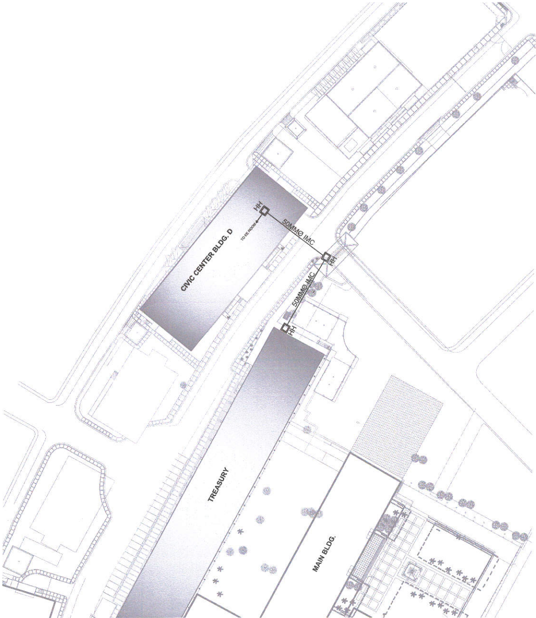
3 SITE DEVELOPMENT PLAN / FEEDER LAYOUT
