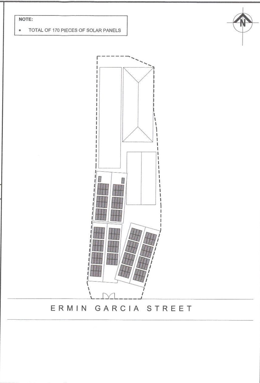
3 SITE DEVELOPMENT PLAN NOT TO SCALE
