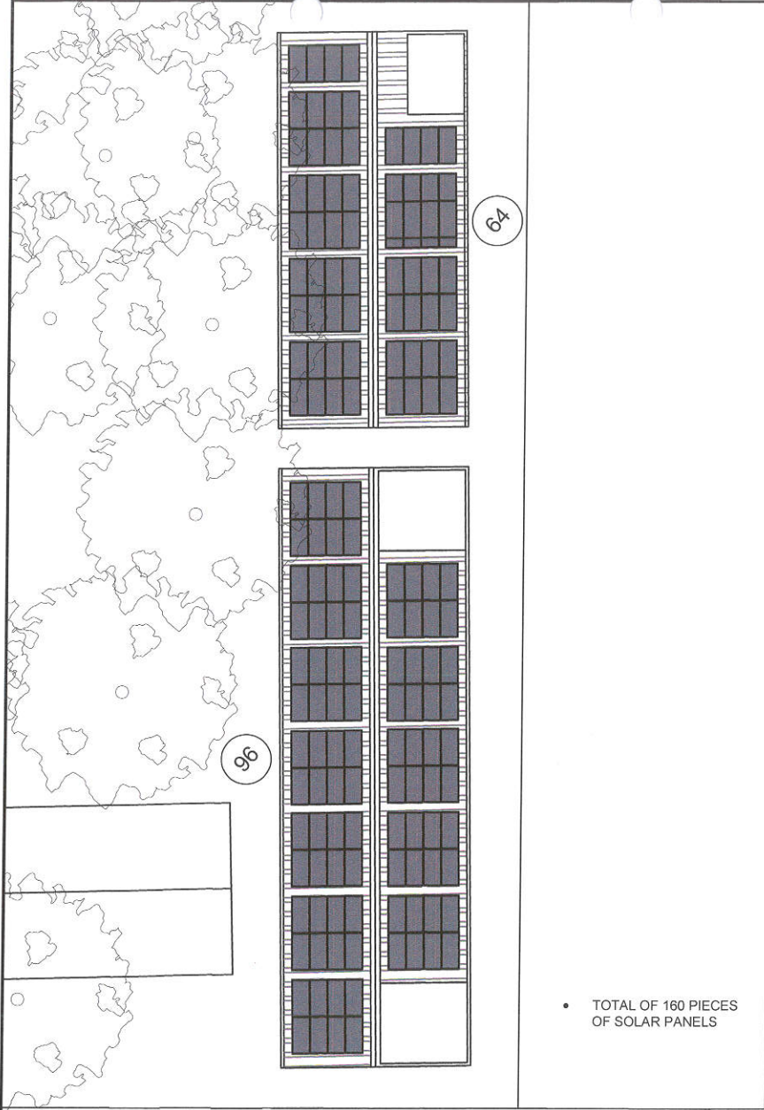
1 ROOF SOLAR PANEL LAYOUT (DIOSDADO P. MACAPAGAL ELEMENTARY SCHOOL)
