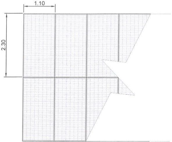
2 SOLAR PANEL PLAN (DIOSDADO P. MACAPAGAL ELEMENTARY SCHOOL)
