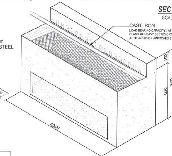
ISOMETRIC SCALE: 1:15MTS
