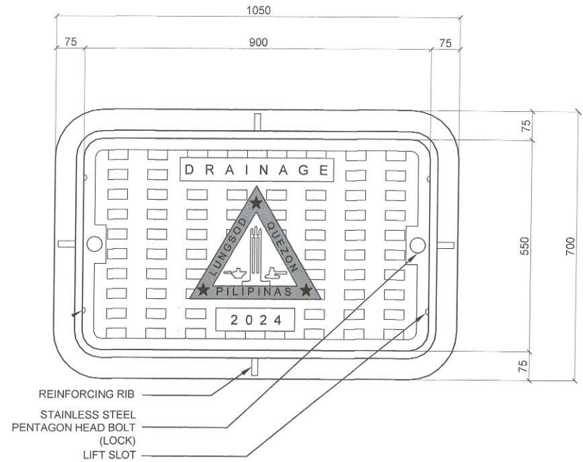
IRON CAST COVER DETAIL SCALE: 1:10MTS
