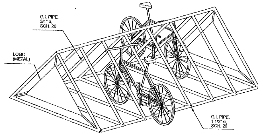
D PERSPECTIVE 03 NOT TO SCALE
