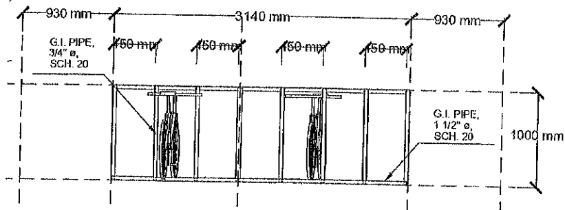
B FRONT ELEVATION 03 NOT TO SCALE
