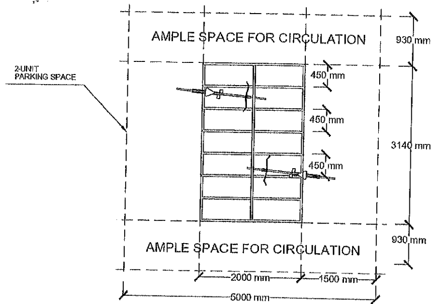
A PLAN VIEW 03 NOT TO SCALE
