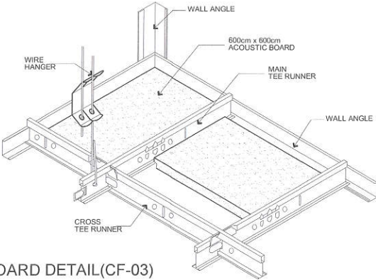
ACOUSTIC BOARD DETAIL(CF-03)
