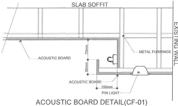
ACOUSTIC BOARD DETAIL(CF-01)
