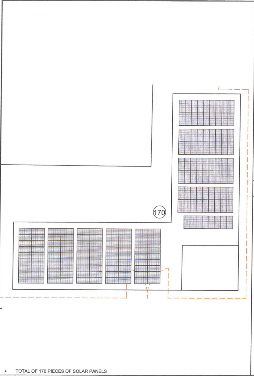
1 ROOF SOLAR PANEL LAYOUT (MANUEL A. ROXAS HIGH SCHOOL) SCALE: NTS
