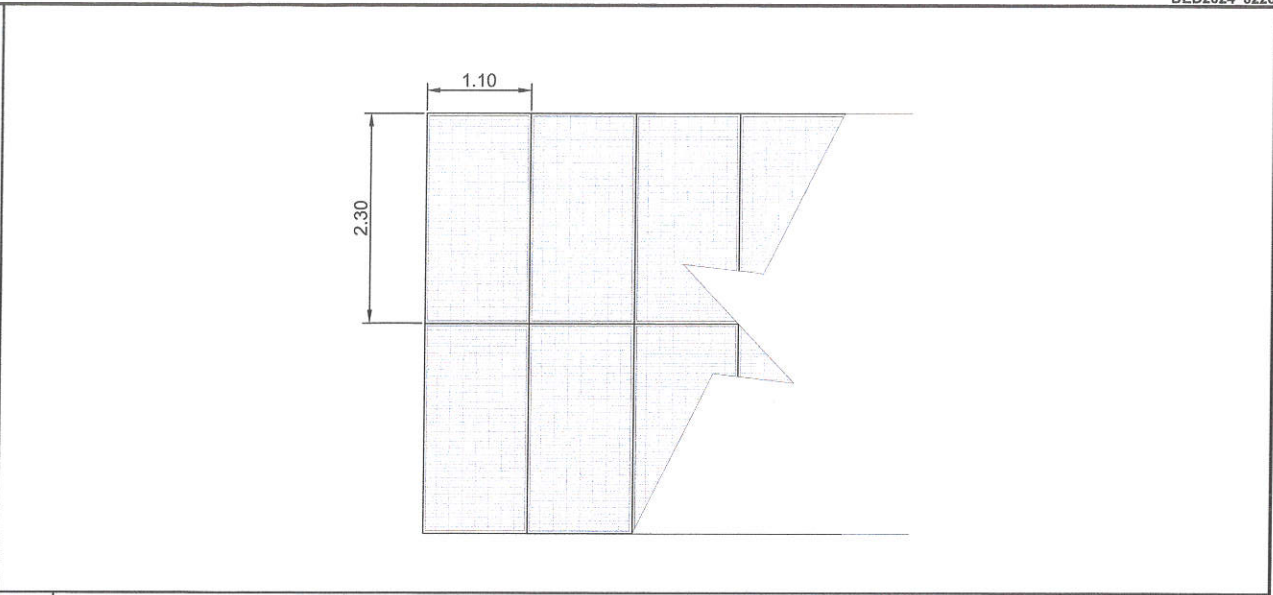
2 SOLAR PANEL PLAN (MANUEL A. ROXAS HIGH SCHOOL) SCALE: NTS
