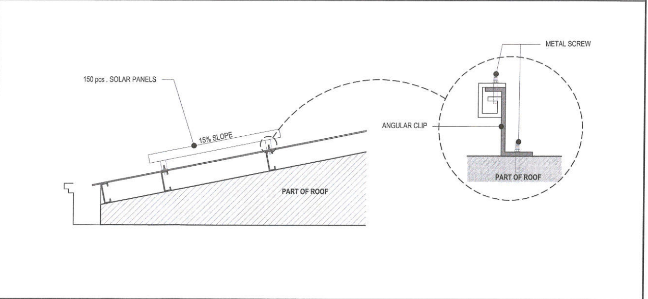
3 SOLAR PANEL DETAIL (MANUEL A. ROXAS HIGH SCHOOL) SCALE: NTS
