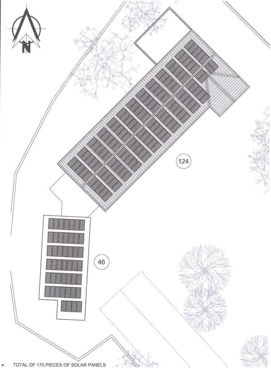
1 ROOF SOLAR PANEL LAYOUT (SAN AGUSTIN ELEMENTARY SCHOOL)
