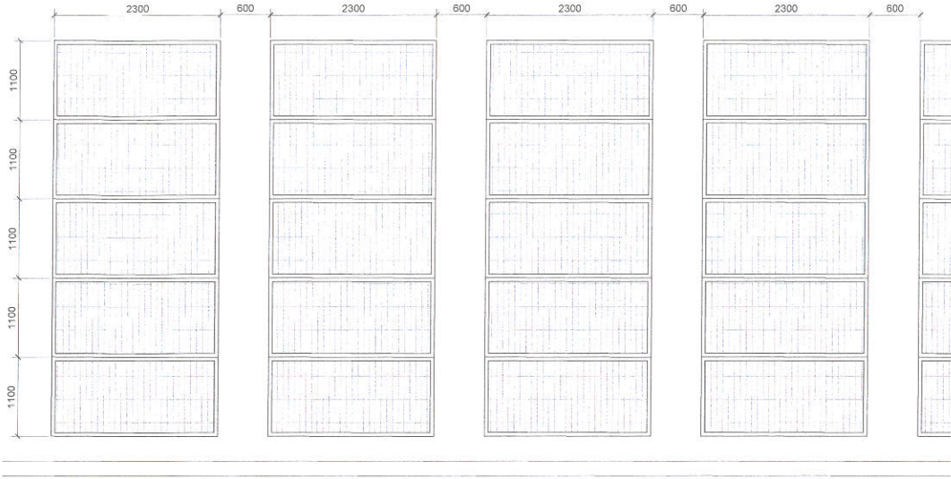
2 SOLAR PANEL PLAN (PLACIDO DEL MUNDO ELEMENTARY SCHOOL )
