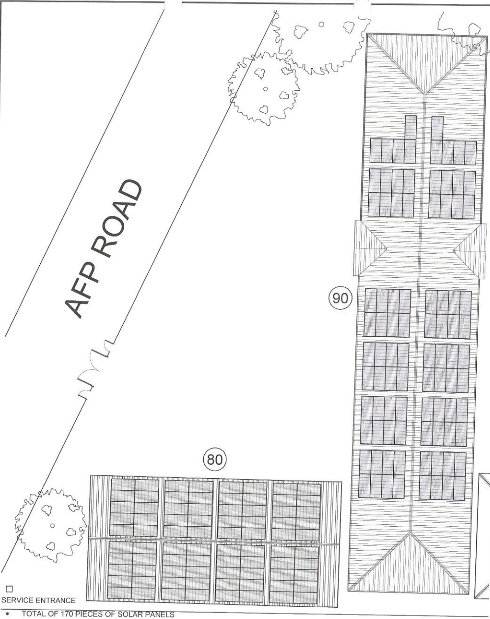
1 ROOF SOLAR PANEL LAYOUT (JUDGE FELICIANO BELMONTE SR. HIGH SCHOOL)
