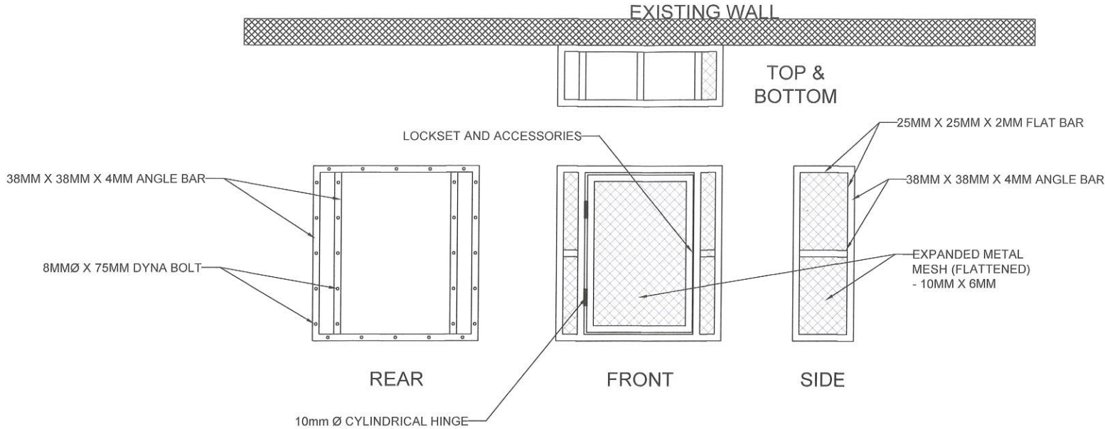
CAGE FOR INVERTER
