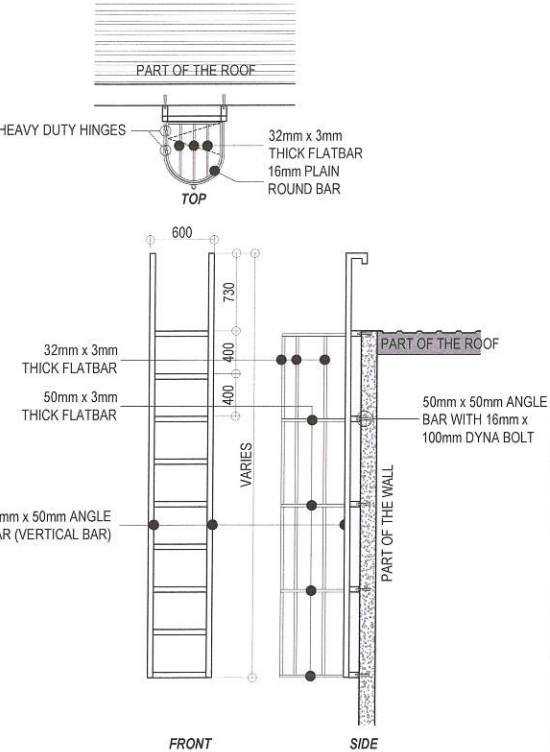
4 ROOF ACCESS "1"
