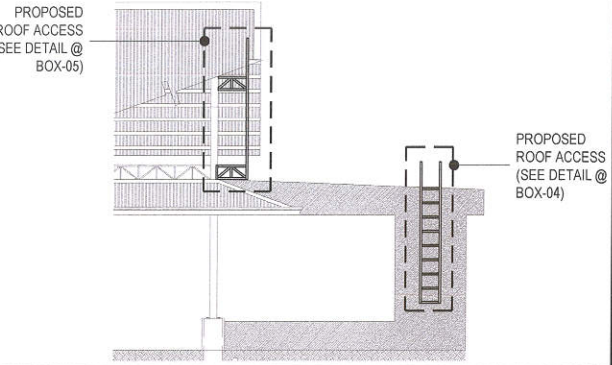
3 ELEVATION "B"
