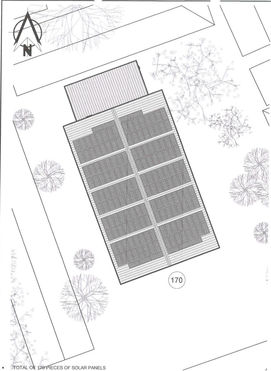
1 ROOF SOLAR PANEL LAYOUT (JUAN SUMULONG HIGH SCHOOL)
