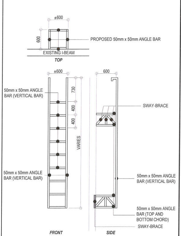
5 ROOF ACCESS "2"
