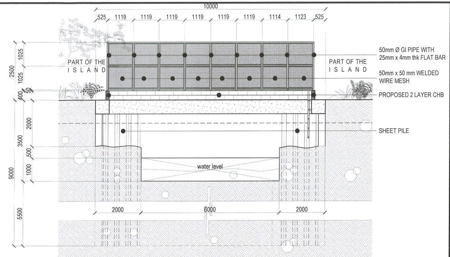
2 SECTION "B"
