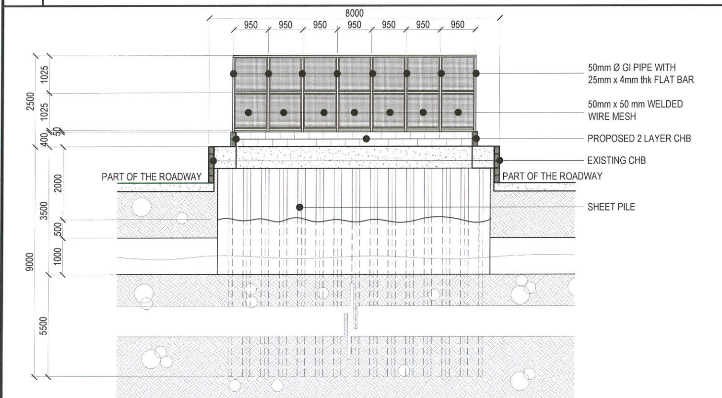
3 SECTION "C"
