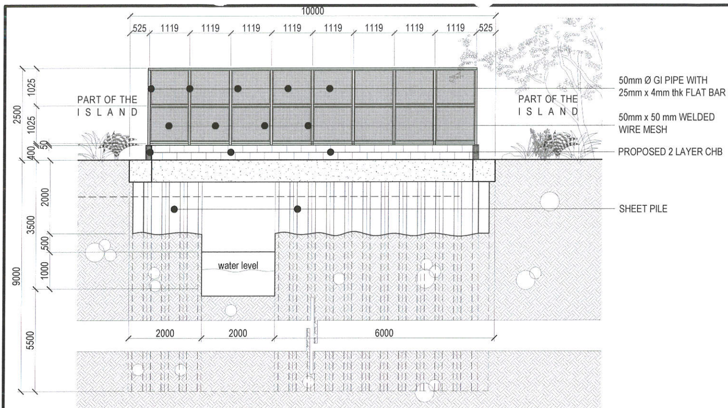
1 SECTION "A"
