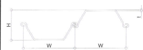
SP-II STEEL SHEET PILING
