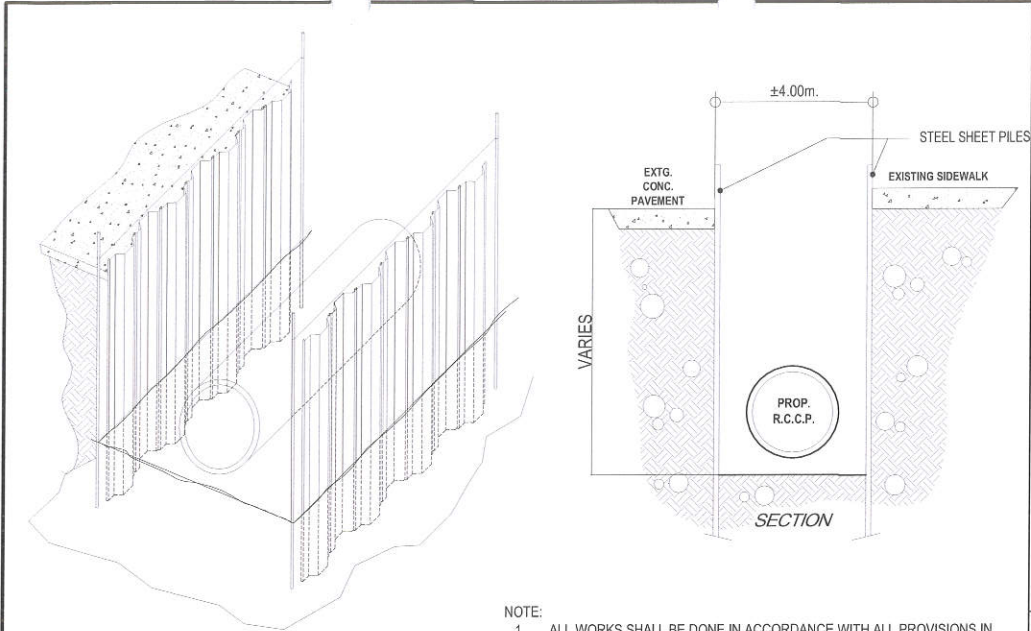
ISOMETRIC VIEW
