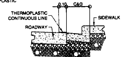
THERMOPLASTIC SECTION
